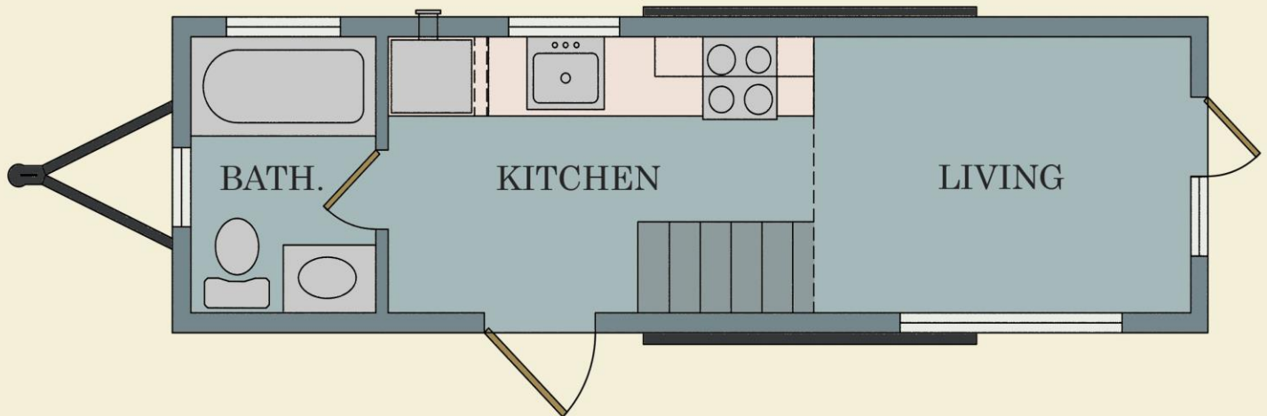
FLOOR PLAN @ 1/4"=1'-0"
