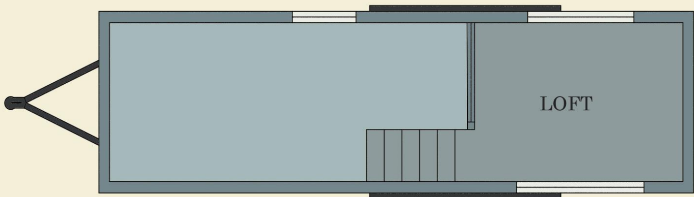
FLOOR PLAN @ 1/4"=1'-0"
